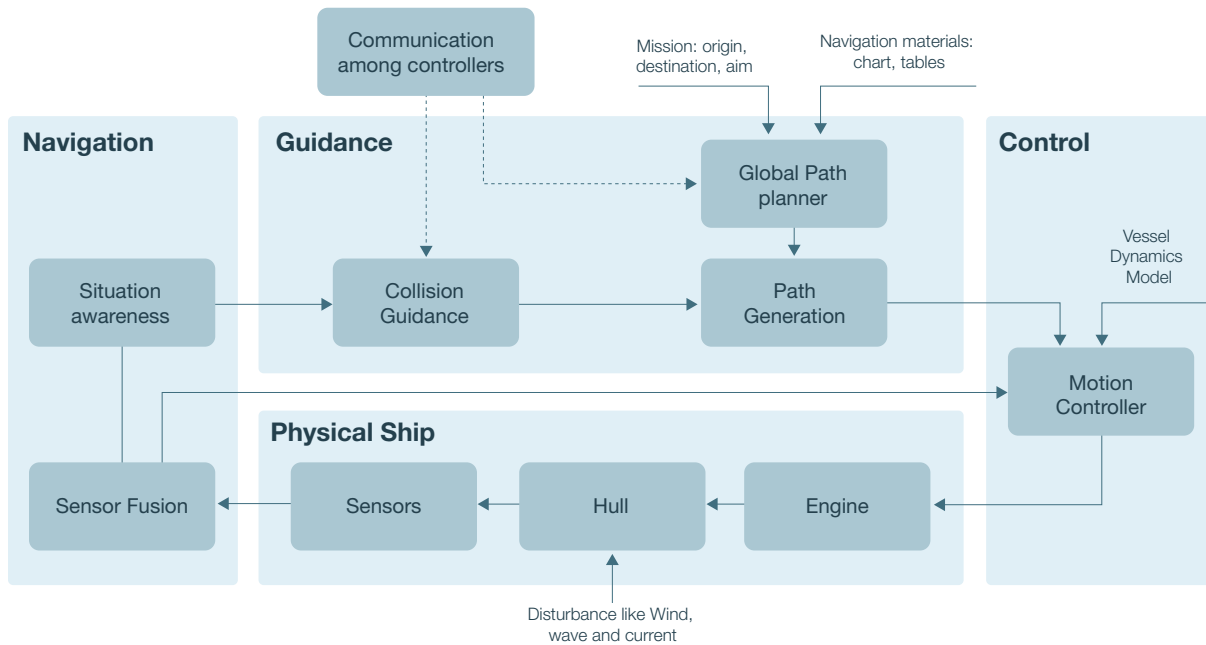
Figure 2 - Parts of an autonomous ship. Figure derived from Schiaretti, Chen & Negenborn (2017) and van Cappelle, Chen & Negenborn (2018)
