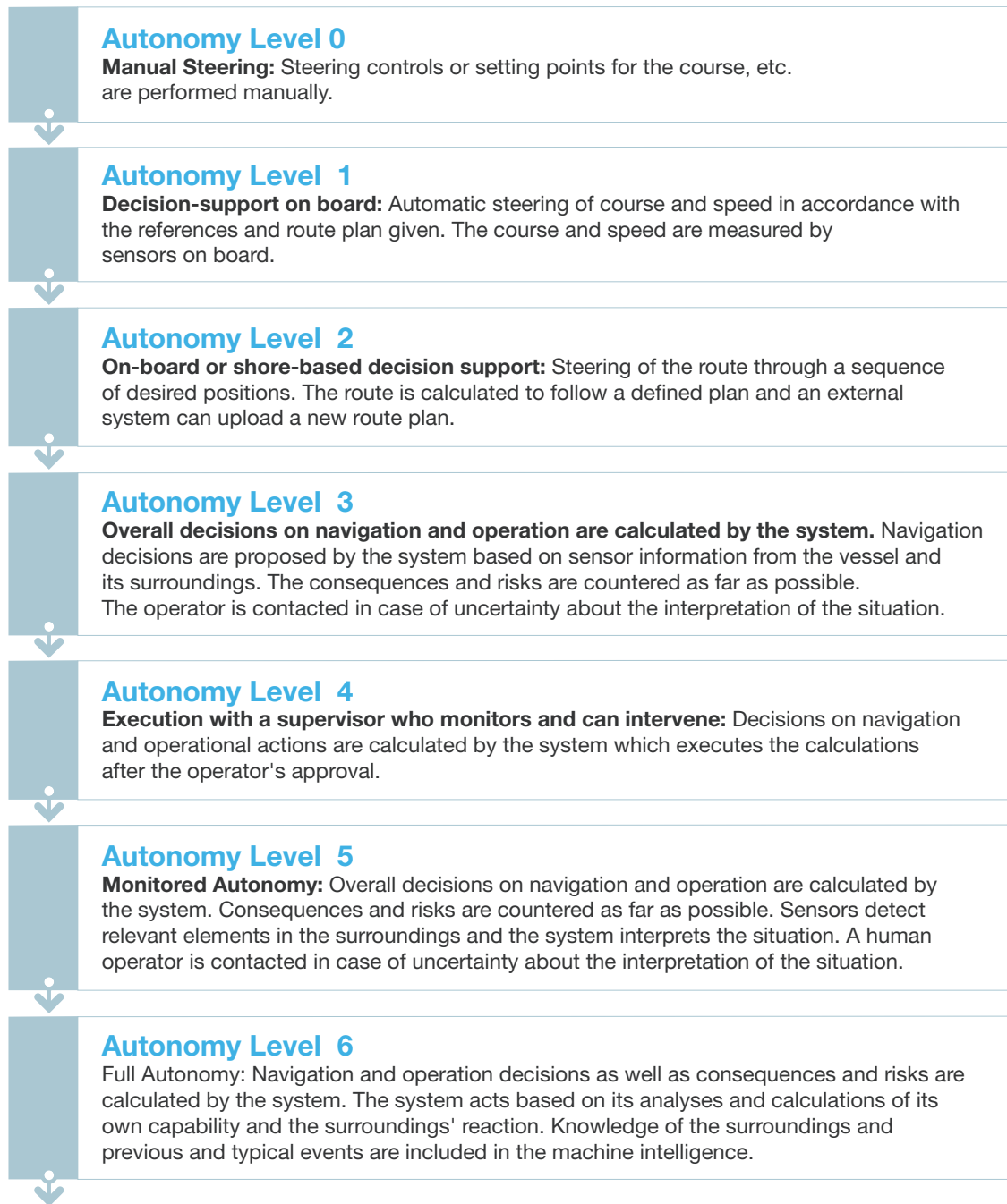
Figure 3: Levels of autonomy (Blanke, Henriques, & Bang, 2017)
