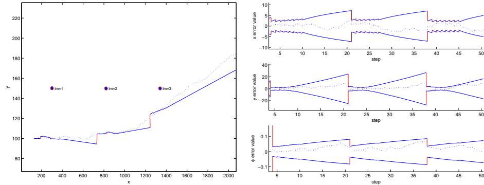
(a) True (dotted, blue), predicted (solid, blue) and corrected (solid, red) trajectory of robot driving with unique landmark identification. The robot senses three landmarks.
