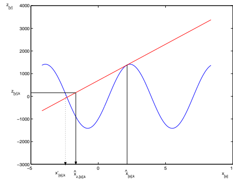
(d) With a different true state, x'_{[\phi],k} , giving the same true measurement z_{[y],k} , the linearization error is smaller, although the estimation error is higher.
