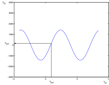
(a) Nonlinear measurement relation between robot's orientation and measured y coordinate. At true orientation x_{[\phi],k} , the robot measures z_{[y],k} .
