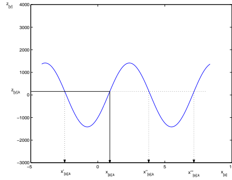
(b) Inverse nonlinear measurement function. The true measurement of z_{[y],k} can have been made from different states: x_{[\phi],k} , x'_{[\phi],k} , etc.
