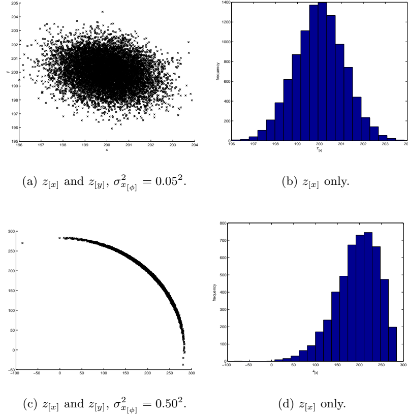
Figure 6.5: Influence of orientation uncertainty on coordinates.
