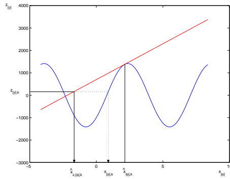
(c) Linearized measurement function at latest state estimate \hat{x}_{[\phi],k} (red) indicating one state from which true measurement z_{[y],k} was made: \hat{x}_{z,[\phi],k} . Notice that this is not the true state from which the measurement was made, x_{[\phi],k} .
